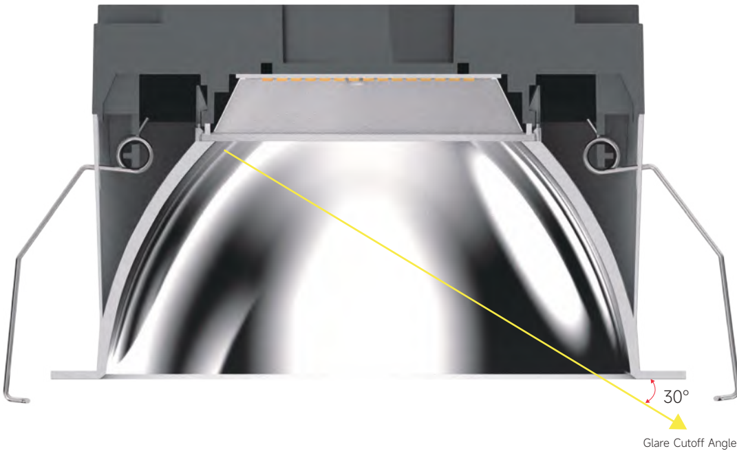
Inner Reflector Surface
