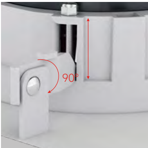
fit for ceiling thickness 1mm to 12mm
