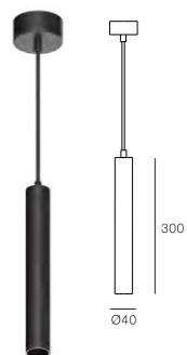
NOVA-P XS 11W 800lm
