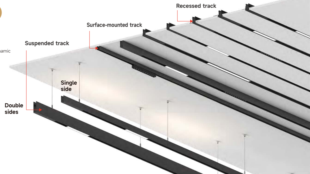
Suspended track
