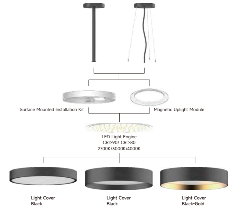
Ceiling Box with Suspension Rod Ceiling Box with Suspension Wires
