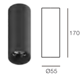
NOVA-C S 11W 720lm-800lm
