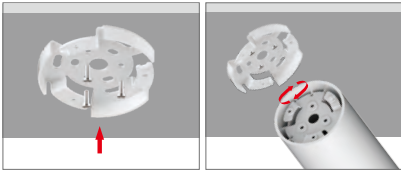
Ceilling installation plate fixed by screws Twist and lock system between housing and ceiling installation plate
